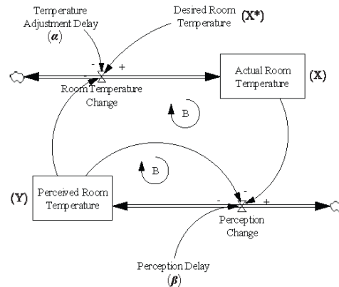
Figure 26. Stock-flow diagram of temperature adjustment model.
