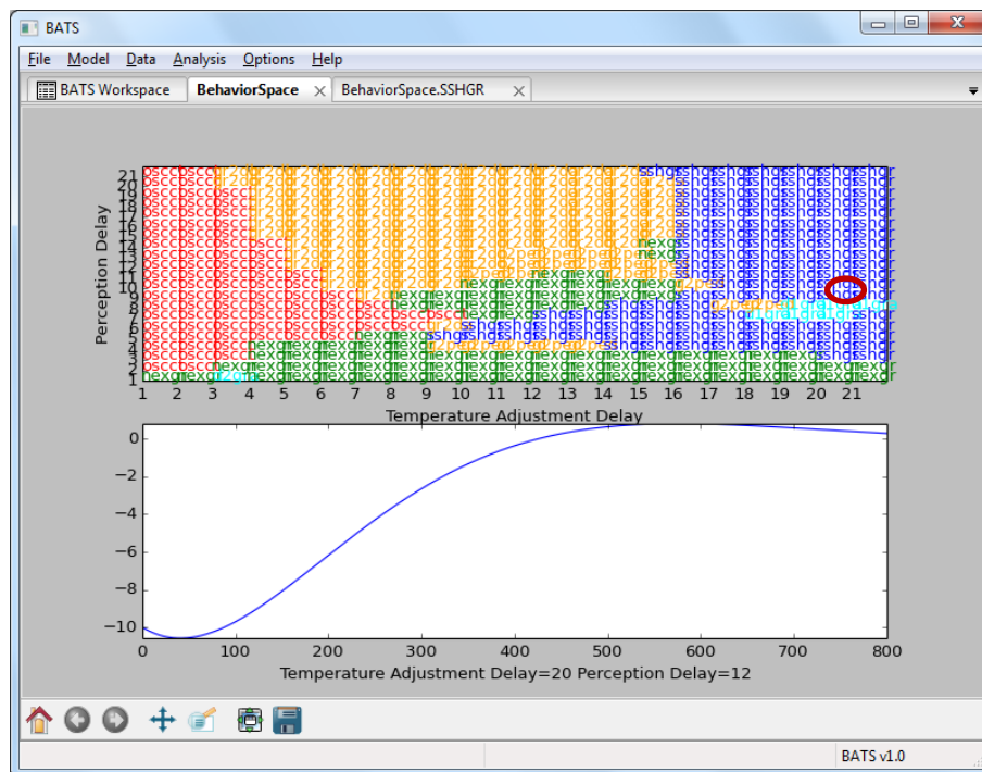
Figure 28. Screenshot for the classifier grid and model behavior plot of Behavior Space Classifier.
