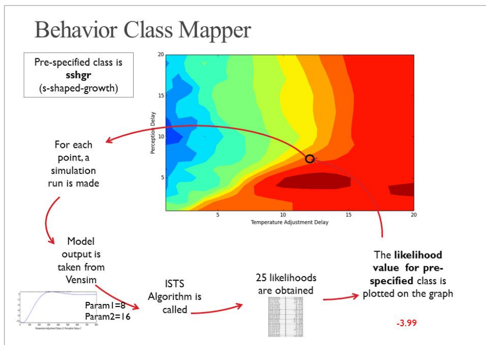
Figure 29. Workflow of Behavior Class Mapper.
