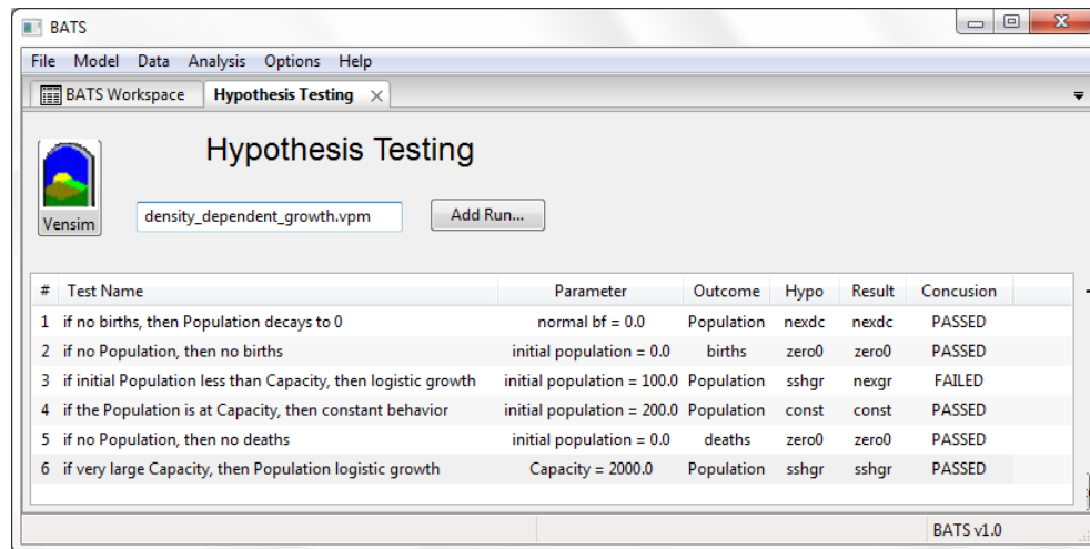
Figure 11. Screenshot for Hypothesis Tester after a representative extreme condition testing process.
