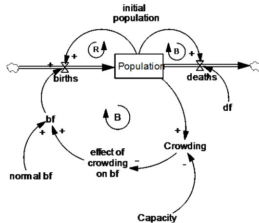
Figure 7. Stock-flow diagram of density-dependent growth model.
