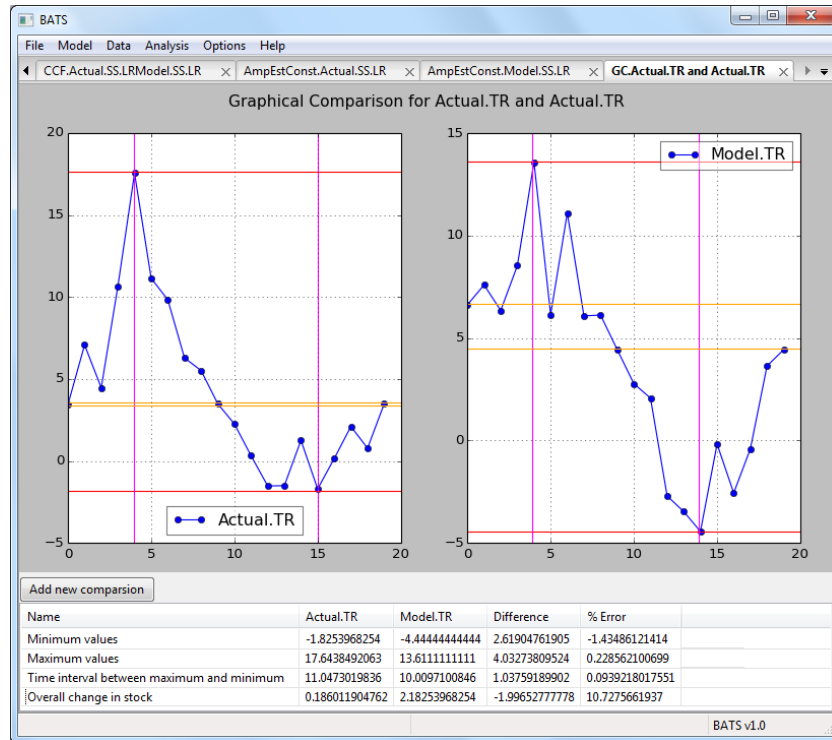
Figure 25. Comparison of transient parts of behaviors and illustration of Graphical Comparison feature.
