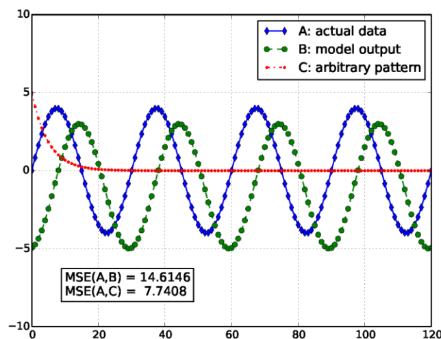
Figure 1. Illustrative example for showing the inappropriateness of MSE.
