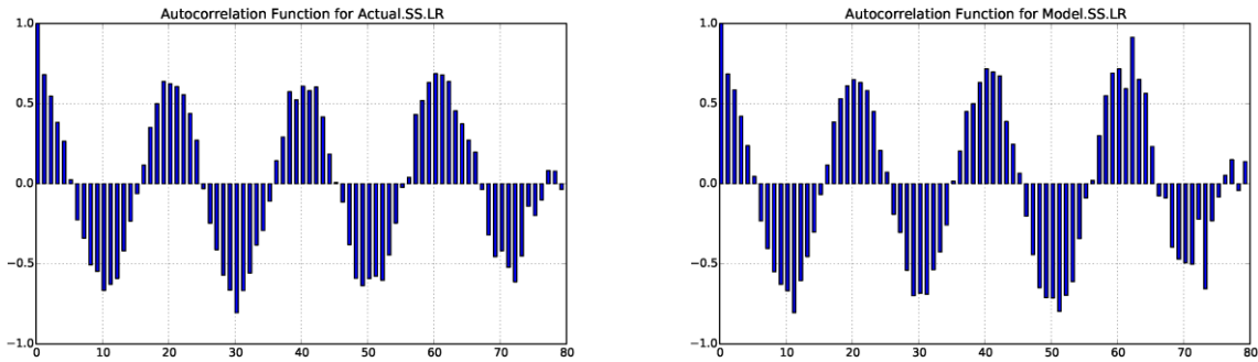
Figure 19. Autocorrelation function results.
