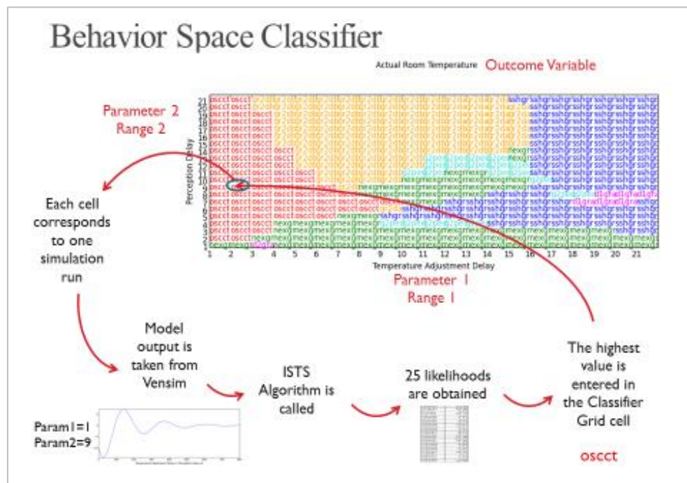
Figure 27. Workflow of Behavior Space Classifier.
