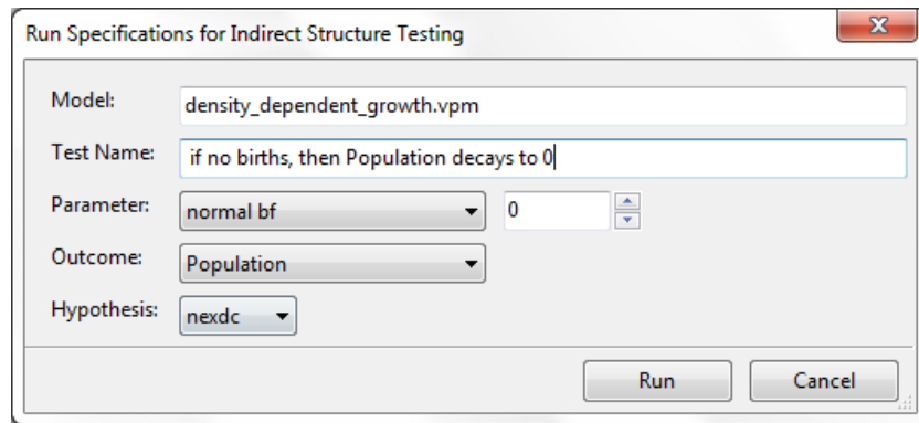
Figure 9. Settings dialog box for Hypothesis Tester feature.
