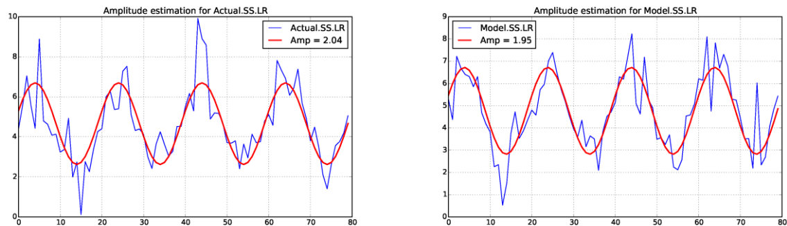
Figure 22. Amplitude estimation using trigonometric function fitting.
