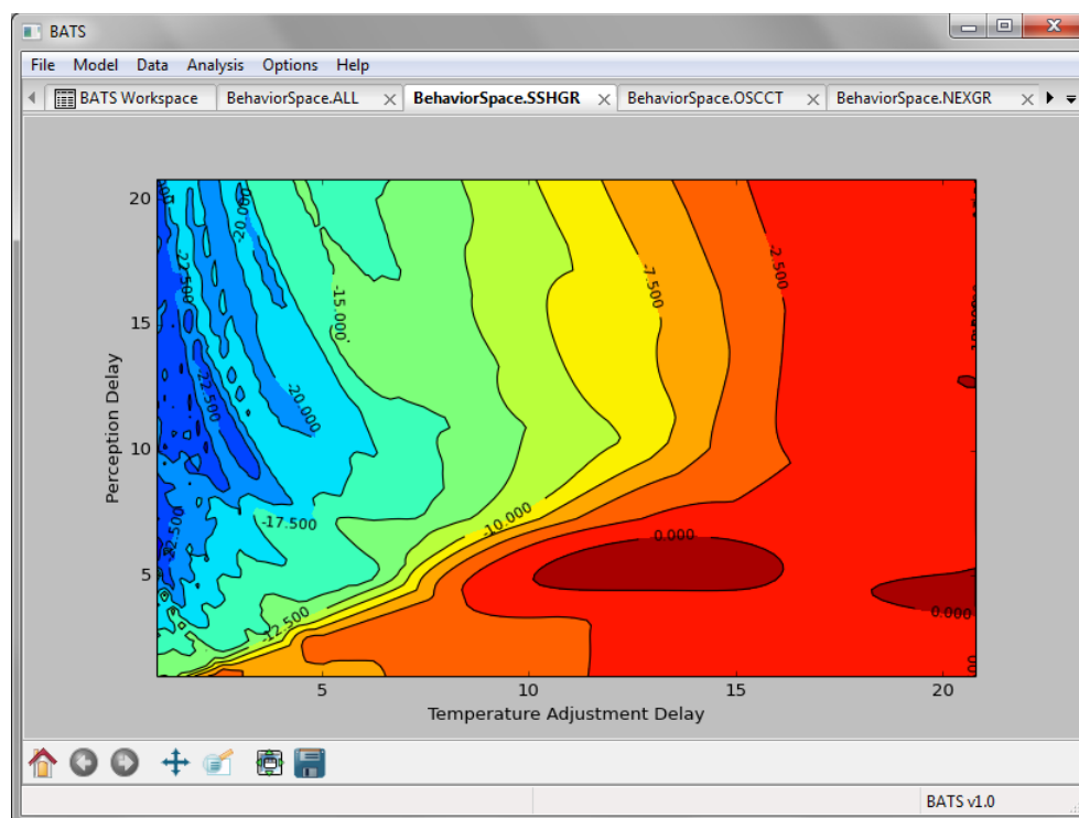
Figure 30. Screenshot for the resulting contour plot of Behavior Class Mapper.
