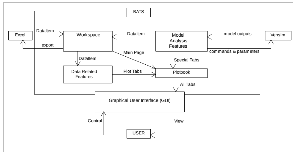
Figure 6. Communication capabilities with external software and internal operations of BATS.
